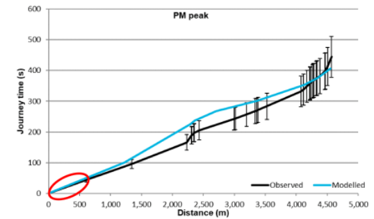
Figure 14: Modelled and Observed Journey Time, A505 Hatters Way Westbound PM peak
